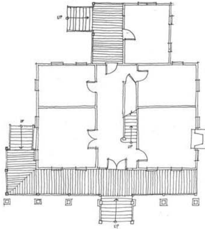
EARLY FLORIDA VERNACULAR HOUSE
