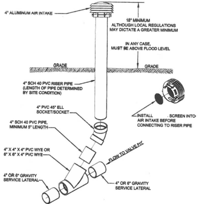
Candy Cane-Style Air Intake Gas Vent Cap-Style Air Intake
